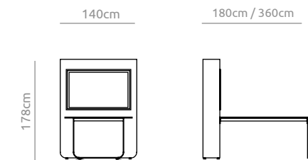
Media table steel leg Low
