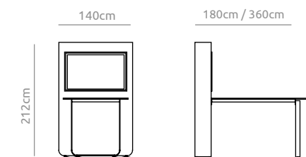
Media table steel leg High
