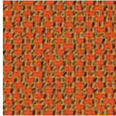
DANTE Cat. Extra Colors 24
