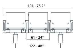
Curved wood seat
