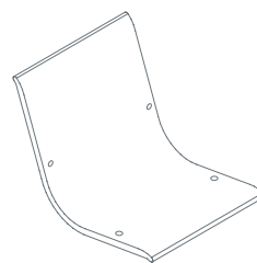
Curved wood shell 1RS5551: L 52 D 65 H 48
