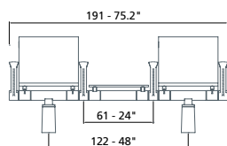
Leather seat with table
