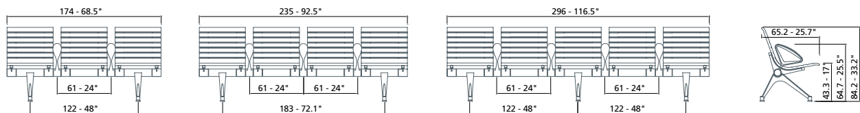
Aluminium backrest seat with armrest and mobile base
