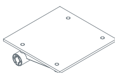
Black laminate table 1RS1511FL: L 52 D 52 H 1,5
