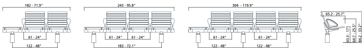
Aluminium backrest seat with table
