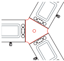
"Y" shaped connector for backbones 1BE0255: L 48 D 54,5 H 53
