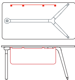
Modesty panel for rectangular workstation 1BE0156: L 100 D 5 H 37
