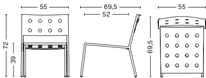
BALCONY LOUNGE CHAIR WIDTH 55 CM | 21.65" DEPTH 69,5 CM | 27.36" HEIGHT 72 CM | 28.35" SEAT HEIGHT 39 CM | 15.35" SEAT DEPTH 52 CM | 20.47"
